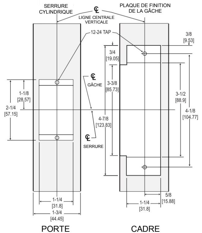
FIGURE 3 : INSTALLATION CADRE
